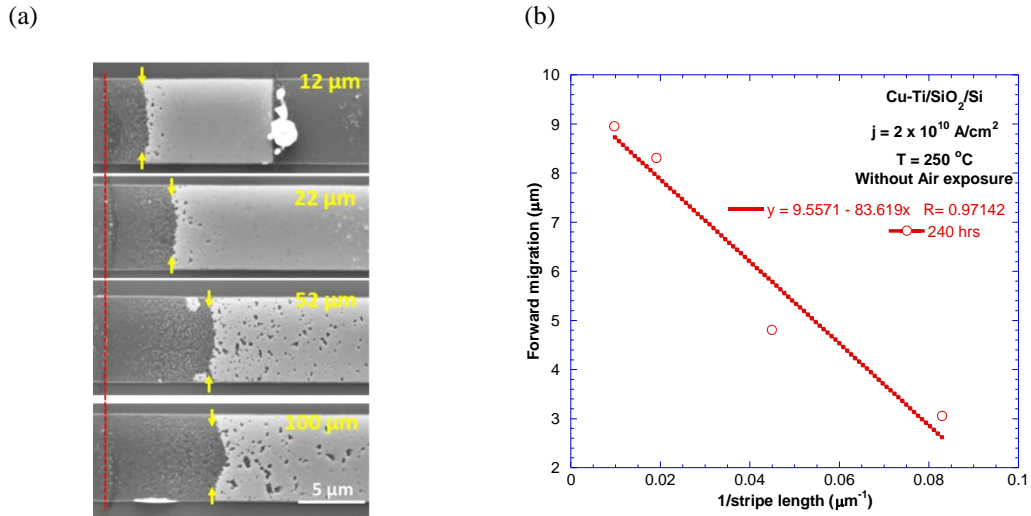
Figure 3: (a) SEM micrographs of Cu films in Cu-Ti system showing region near the cathode after 14,400 min (or 240 h) of electric current loading. The red broken vertical line shows the initial location of the Cu film, whereas the yellow vertical arrows in each stripe show the end of the Cu film after the test. (b) Variation of the forward migration or the extent of the depletion zone at the cathode as function of the inverse of the stripe length. The open symbols are the datum points, whereas the broken lines are the best fit curves. Equation for the best fit curve, along with the curve fitting parameters are shown in the legend.
