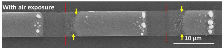
Figure 4: (a) Representative SEM micrograph showing Cu film in Cu-Ti-Si system (with Ti exposed to air for a few seconds prior to deposition of Cu) after passage of electric current of nominal density of 2 \times 10^{10} A/m 2 at 250 °C for 1500 min. Red broken vertical line shows the initial location of the Cu film, whereas yellow vertical arrow shows the end of the Cu film after the test. (b) Variation of extent of the depletion zone at anode as function of inverse of the stripe length.
