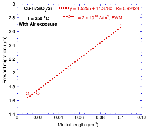
Figure 4: (a) Representative SEM micrograph showing Cu film in Cu-Ti-Si system (with Ti exposed to air for a few seconds prior to deposition of Cu) after passage of electric current of nominal density of 2 \times 10^{10} A/m 2 at 250 °C for 1500 min. Red broken vertical line shows the initial location of the Cu film, whereas yellow vertical arrow shows the end of the Cu film after the test. (b) Variation of extent of the depletion zone at anode as function of inverse of the stripe length.
